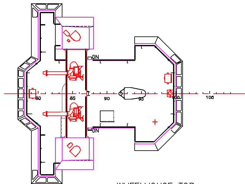
WHEELHOUSE TOP
