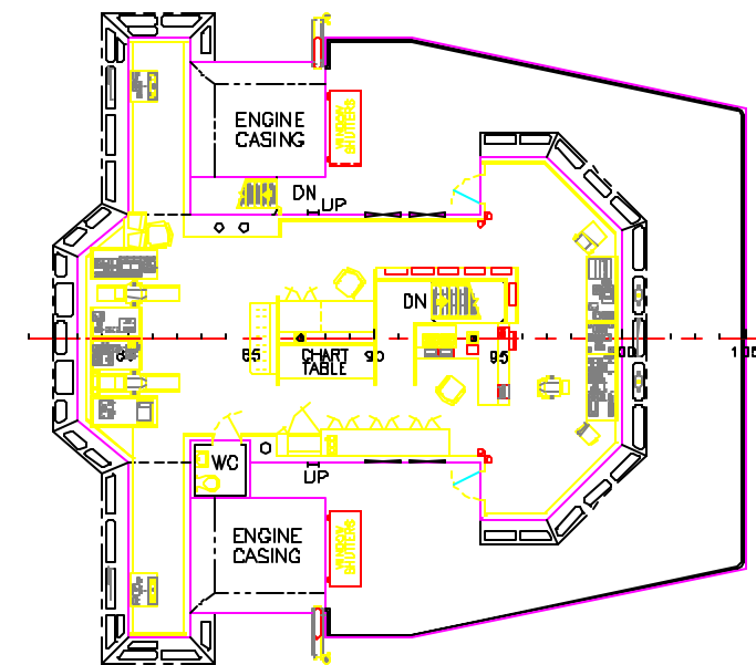
NAVIGATING BRIDGE
